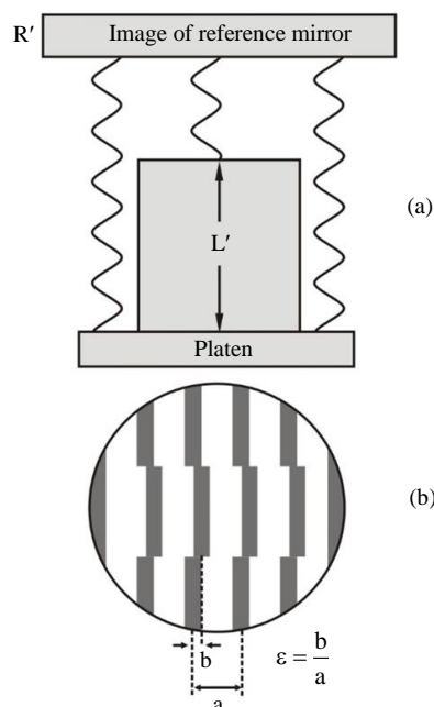
Fig. 2: (a) Depiction of the incidence light to the top of the gauge block and the top surface of platen and (b) observed interference fringes
