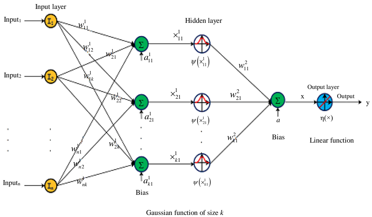
Fig. 2: The RBF architectural model
